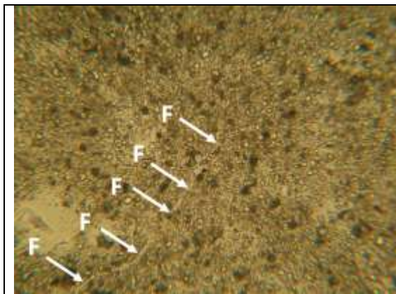
Fig. 5. Detail of the terminal area of a crack; In the upper part of the image the crack does not continue in the section plane (400x).
